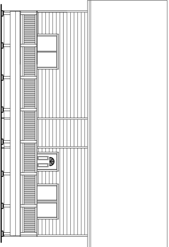
1 BACK ELEVATION 1/4" = 1'-0"
