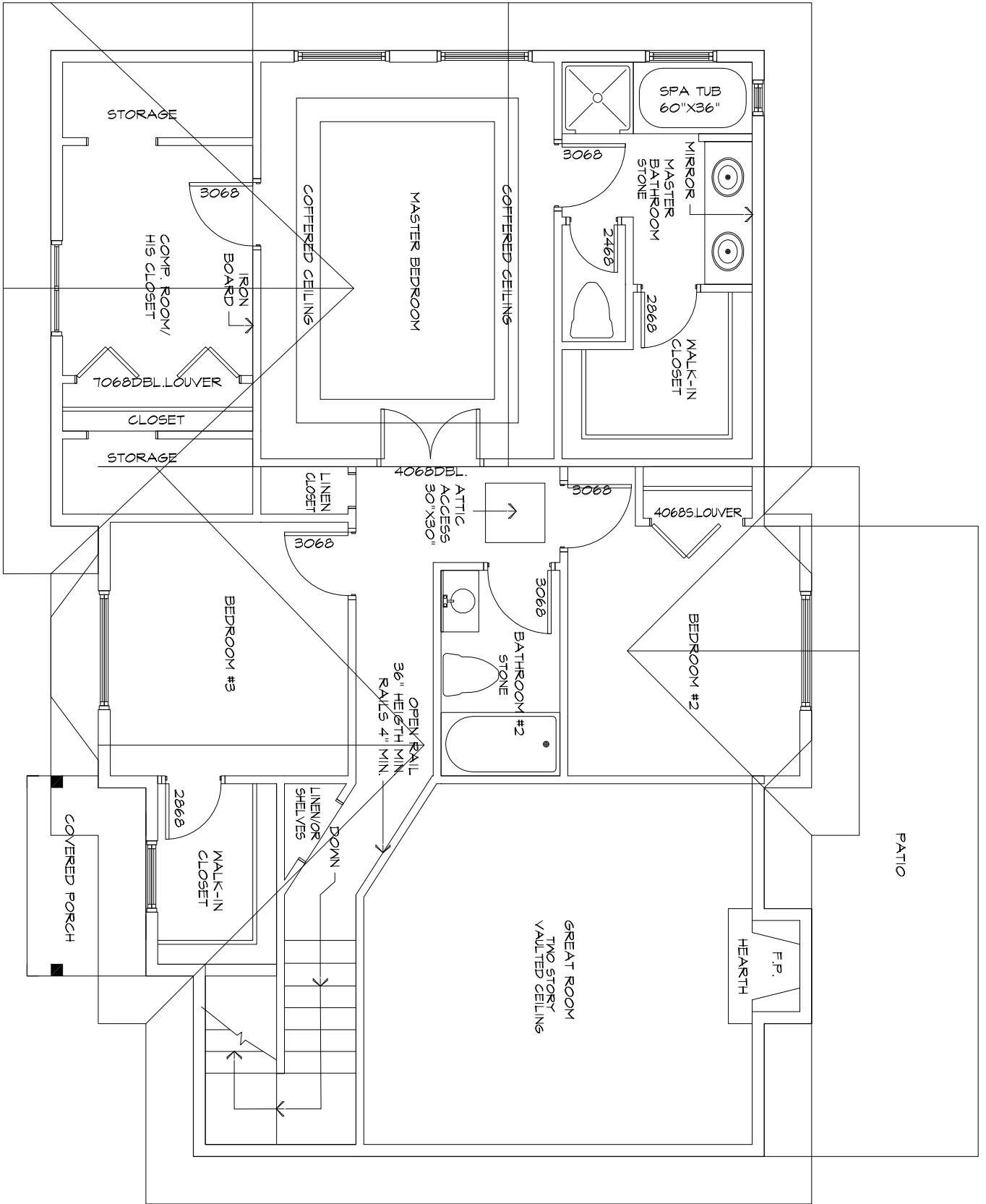
1 UPPER FLOOR PLAN 1/4" = 1'-0" 1,063 SQ. FT.
